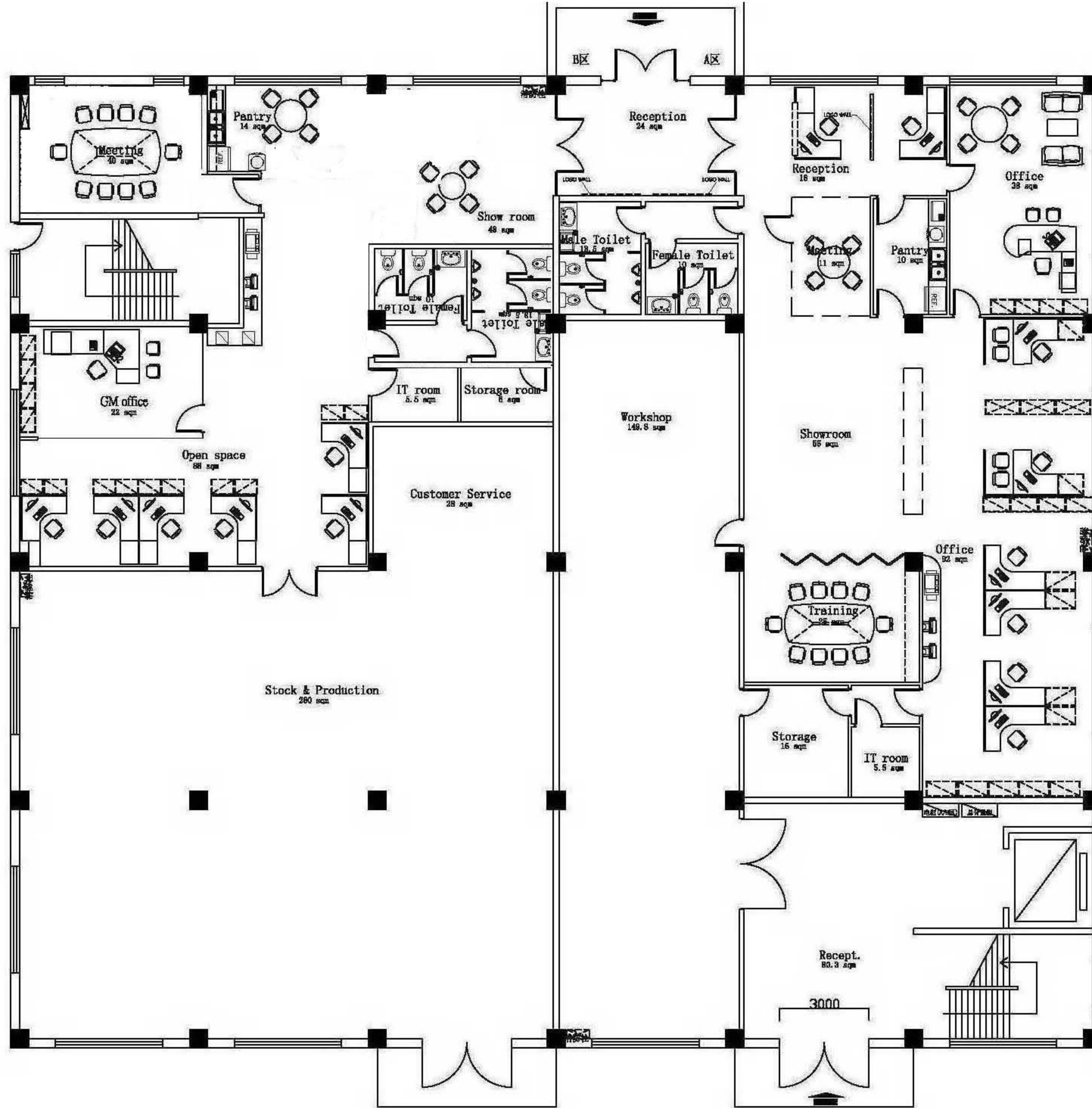
Layout (Section A/B) of the SCS Machinery Center (Building No.1)
